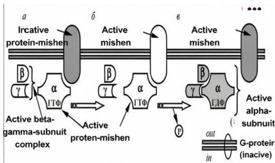
Figure 5.1: Activation of G-protein: a-b – intermediate stages of the process
