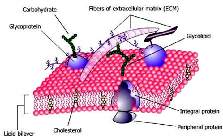
Figure 3: Cellular Membranes
